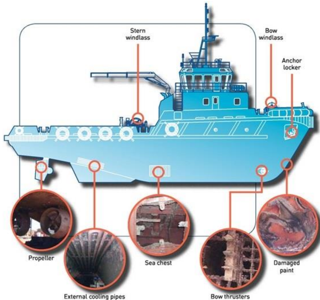
Figure 2 Niche areas where biofouling can accumulate on a non-trading vessel
