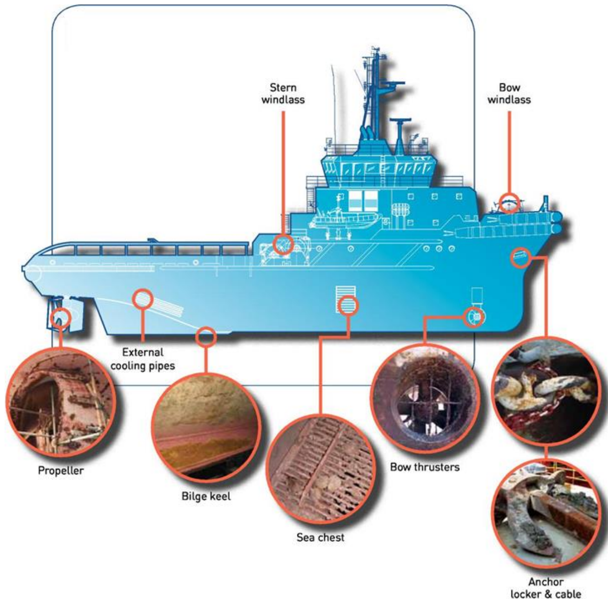
Figure 2 Niche areas where biofouling can accumulate on a petroleum vessel
