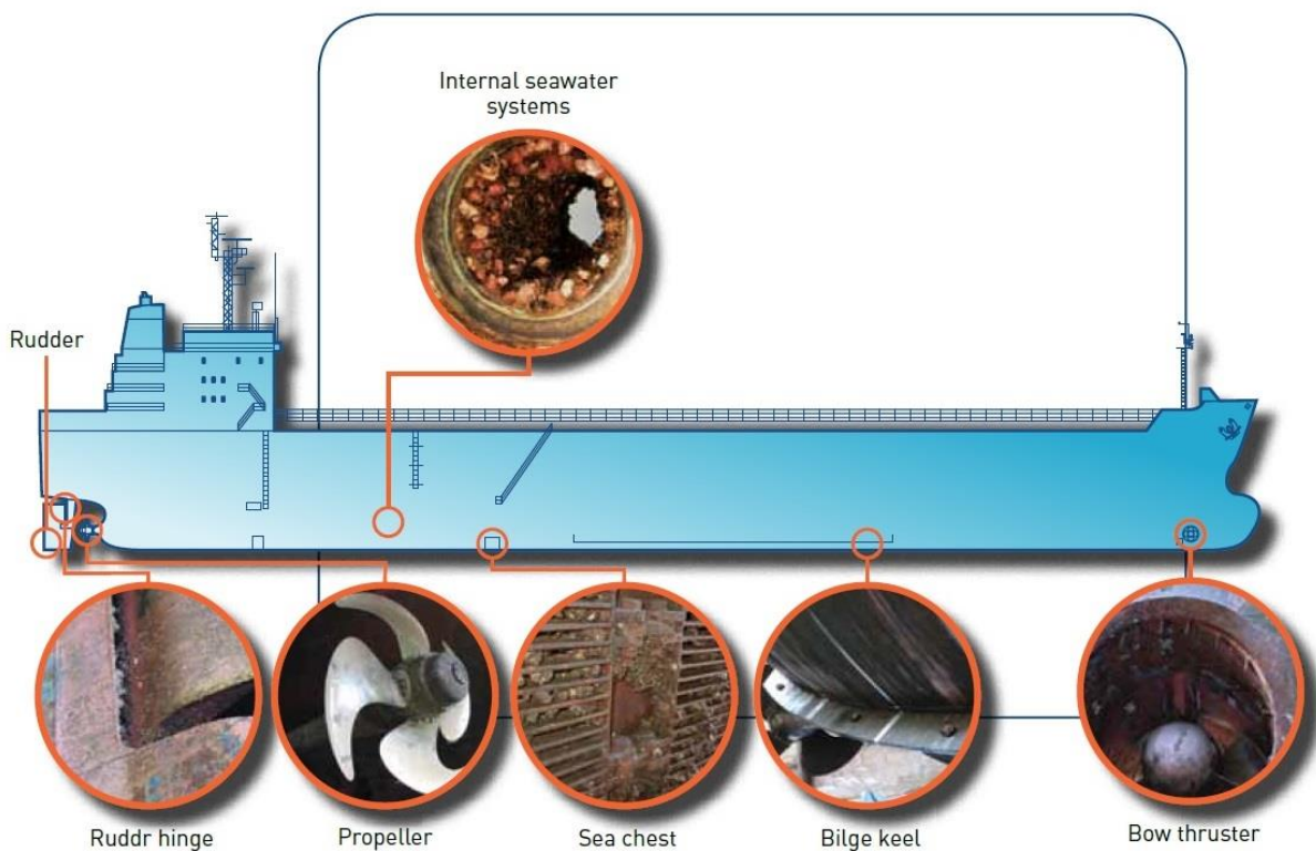
Figure 1 Niche areas where biofouling can accumulate on a commercial vessel
